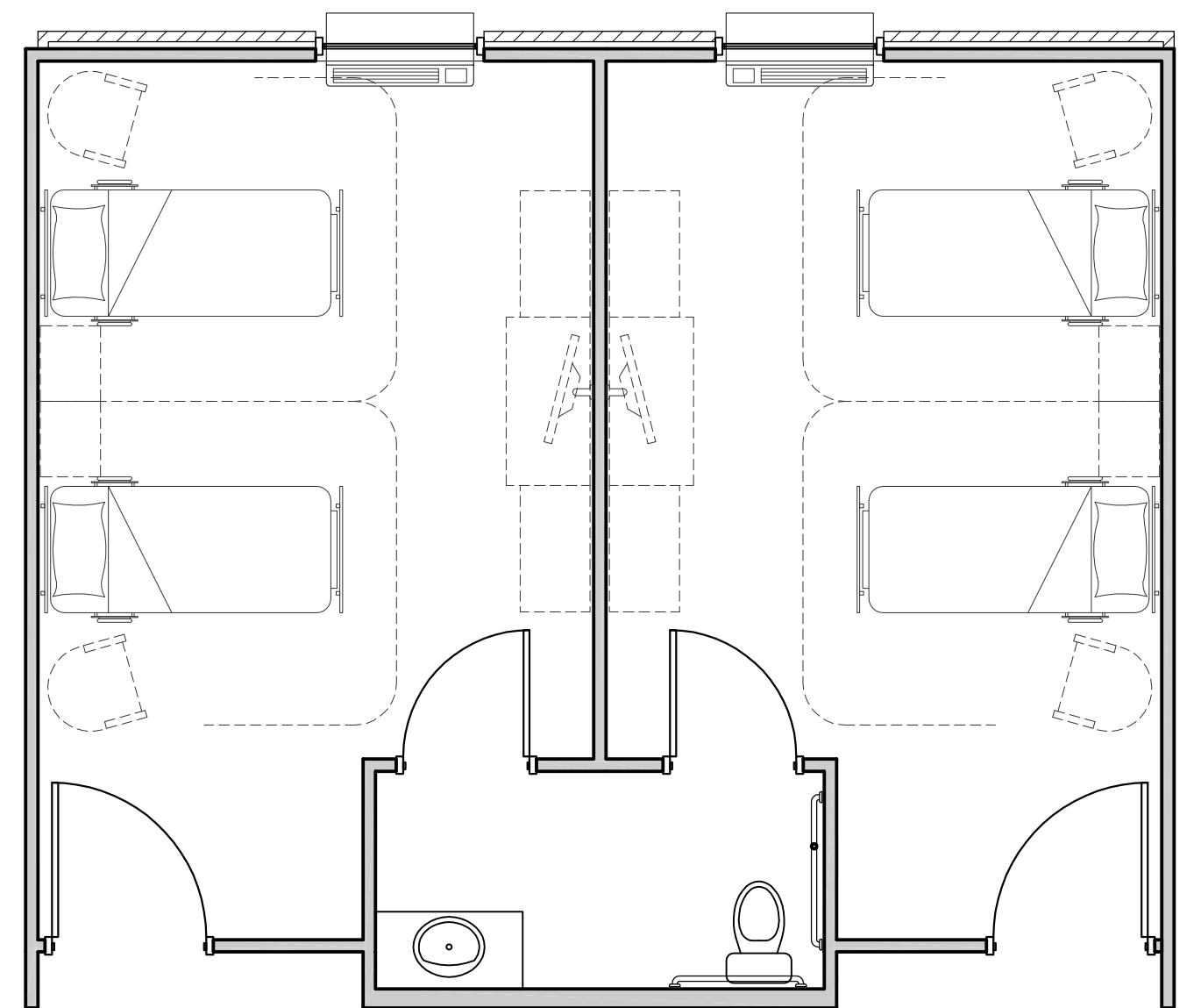
CLASS B ROOMS DOUBLE OCCUPANCY DOUBLE LICENCE SHARED BATHROOM W/ 1 ADJACENT ROOM BATHROOM SHALL HAVE TOILET, SINK, CABINET & MIRROR
