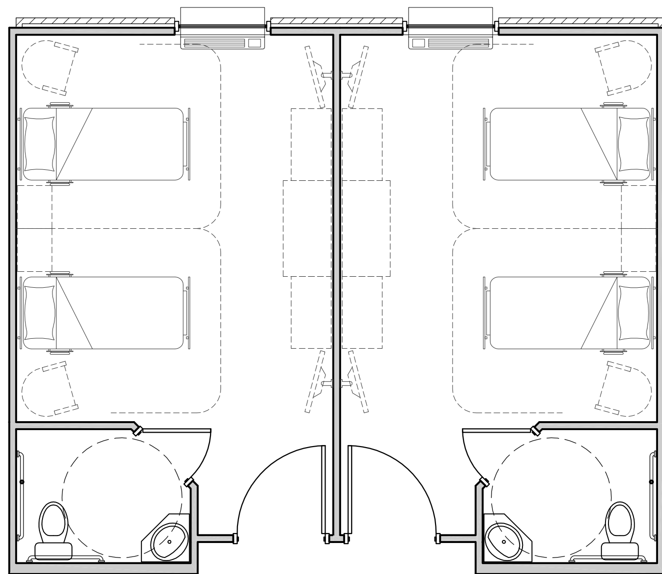
CLASS B ROOM DOUBLE OCCUPANCY DOUBLE LICENCE BATHROOM SHALL HAVE TOILET, SINK, CABINET & MIRROR
